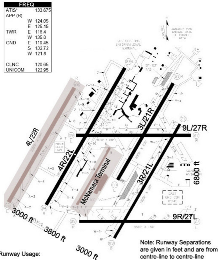
Fig.1: Airfield Layout Plan of DTW showing the New Runway 4L/22R and McNamara Terminal for NWA
